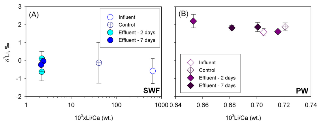
Fig. 5. Variation in \delta^7\text{Li} vs. 1000 \times \text{Li}/\text{Ca} of experiments SWF (A) and experiments PW (B). These figures show that carbonate dissolution and desorption of Li from exchange sites negligibly affect Li concentration and \delta^7\text{Li} in the reacted fluids.
