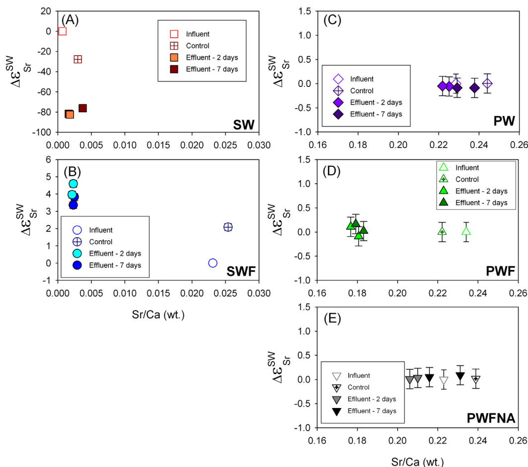
Fig. 4. Variation in \Delta\epsilon_{\text{Sr}}^{\text{SW}} ( \Delta\epsilon_{\text{Sr}}^{\text{SW}} = \epsilon_{\text{SW reacted fluid}}^{\text{Sr}} - \epsilon_{\text{SW initial fluid}}^{\text{Sr}} ) vs. Sr/Ca of all experiments. Error bars in A and B are within the size of the symbols.
